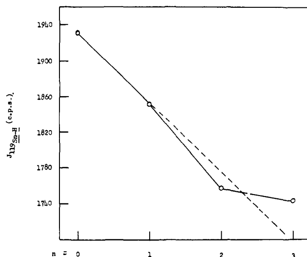
Fig. 1.— J_{119\text{Sn-H}} as a function of n for the series (\text{CH}_3)_n\text{-SnH}_{4-n} . If the substituent effects were additive, the points for n = 2 and n = 3 would have fallen on the extrapolated (dotted) line.
